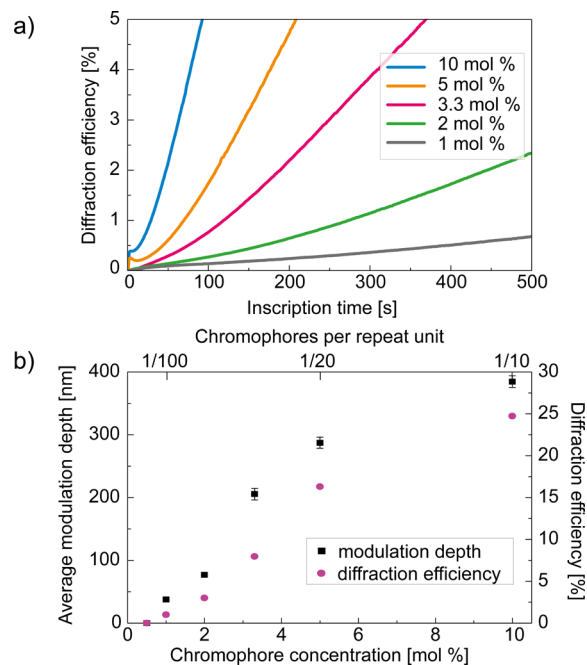
Figure 2. (a) Evolution of diffraction efficiency as a function of inscription time, and (b) average modulation depths (black cubes) and the diffraction efficiencies (violet circles) of the SRGs as a function of chromophore content. The error bars present the standard deviation in the AFM data.
