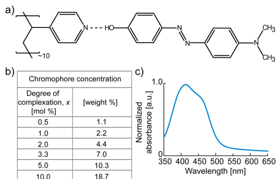
Figure 1. (a) Chemical structure of the nominally stoichiometric complex between P4VP and OH-DMA, (b) the chromophore concentration as weight percentage in the studied complexes, and (c) the normalized UV–vis absorption spectrum of a 10-mol % film.
